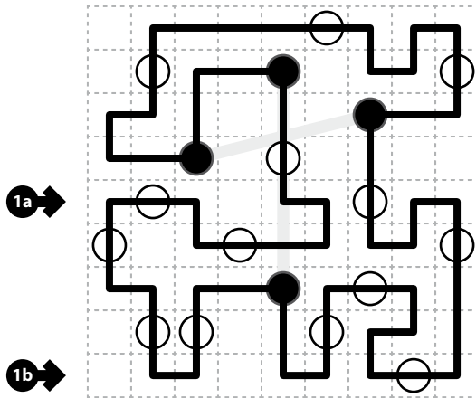
Southern Cross
