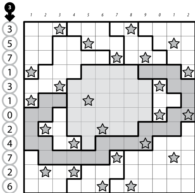
Saturn
