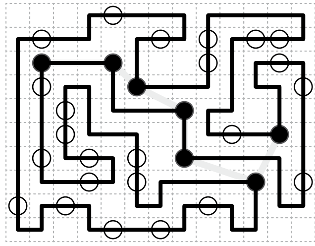
Big Dipper
